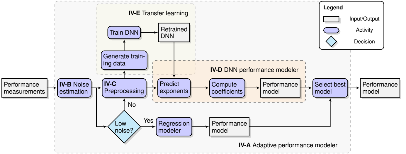
Fig. 1: Flowchart outlining the basic adaptive performance modeling process. The letters (IV-A) reference the paragraphs of the approach where the associated components of the adaptive modeler are described in detail.
