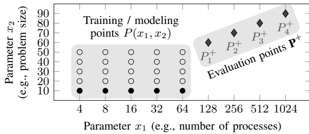
Fig. 2: Performance experiments required for one and two-parameter analysis. The filled black circles represent a list of measurement points P(x_1) using the parameter-value set \mathbf{x}_1 that would be sufficient to generate a single-parameter model for parameter x_1 . All circles represent the measurement points required for a two-parameter model describing how x_1 and x_2 affect performance. The filled diamonds are the measurement points reserved for evaluation.
