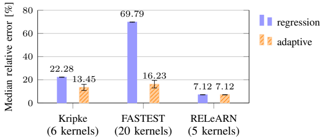
Fig. 4: Comparison of the median relative prediction error in percent of the regression and adaptive modeler for modeling the performance relevant kernels of the case studies. The error bars show the 99% confidence intervals of the reported median relative error.
