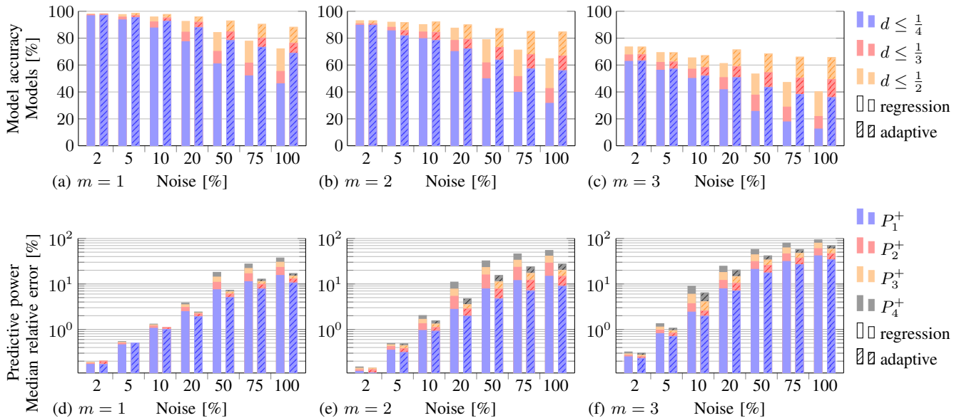
Fig. 3: Comparison of the model accuracy and predictive power of the regression and adaptive modeler for different numbers of parameters m = 1, 2, 3 and noise levels n = 2\%, 5\%, 10\%, 20\%, 50\%, 75\%, 100\% . The Figures (a), (b), and (c) outline the percentage of models where the distance of the lead exponents d is smaller as or equal to \frac{1}{4} , \frac{1}{3} , or \frac{1}{2} when compared to the synthetic baseline. The smaller the distance, the more accurate the performance model. The Figures (d), (e), and (f) show the median relative prediction error in percent for the four evaluation points \mathbf{P}^+ when compared to the synthetic baseline. The higher the error the lower the predictive power of the models.
