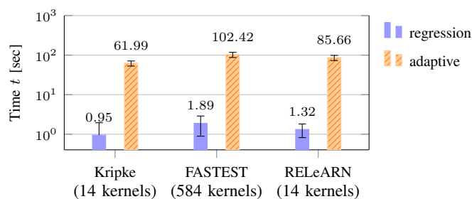
Fig. 6: Comparison of the amount of time t in seconds required by the regression and adaptive modeler for modeling the main kernels of the application case studies. The error bars show the 99% confidence intervals of the reported time.
