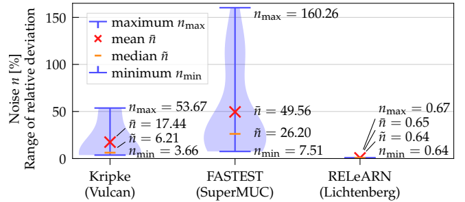
Fig. 5: Noise-level distributions of the performance measurements of the application case studies.
