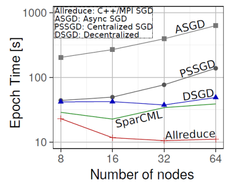
(a) Strong scaling (Wide ResNet 28x10). Fig. 11: Scaling Analysis of Level 3
