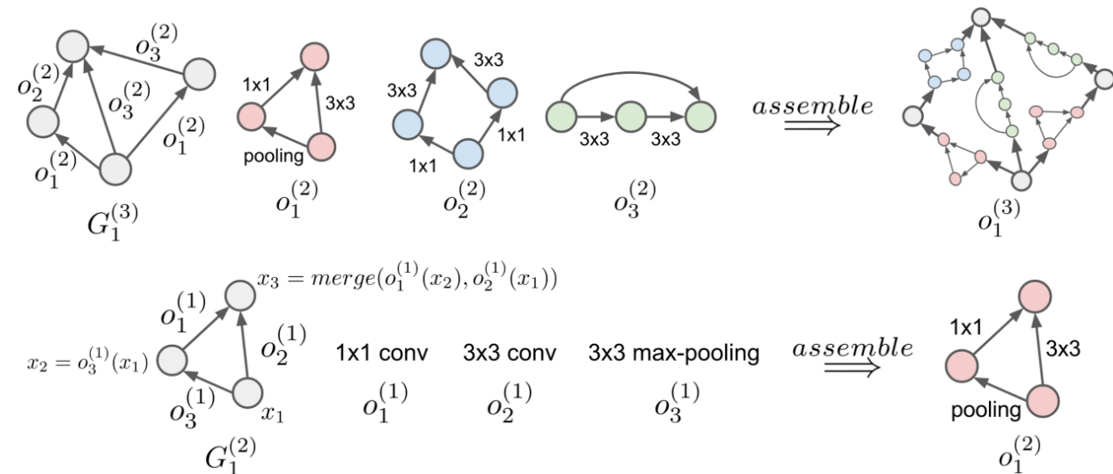
Evolutionary Algorithms [4]
